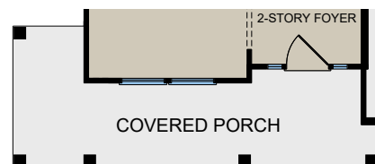
Optional Wrap Around Porch Elevation C
