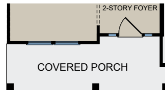
Partial First Floor Elevation C
