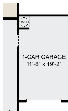
Optional 1 Car Garage
